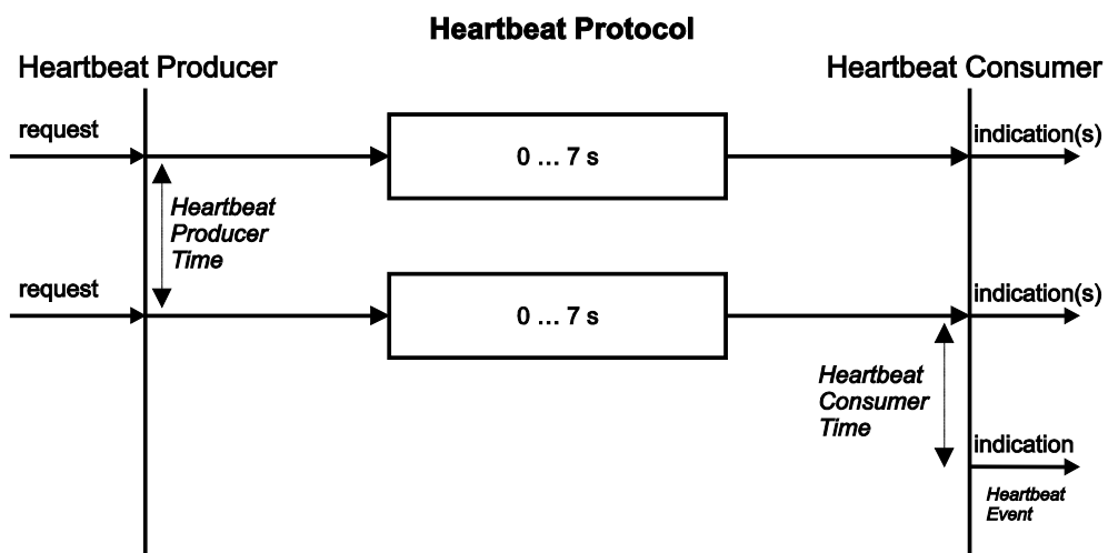
Figure 66: Heartbeat Protocol
