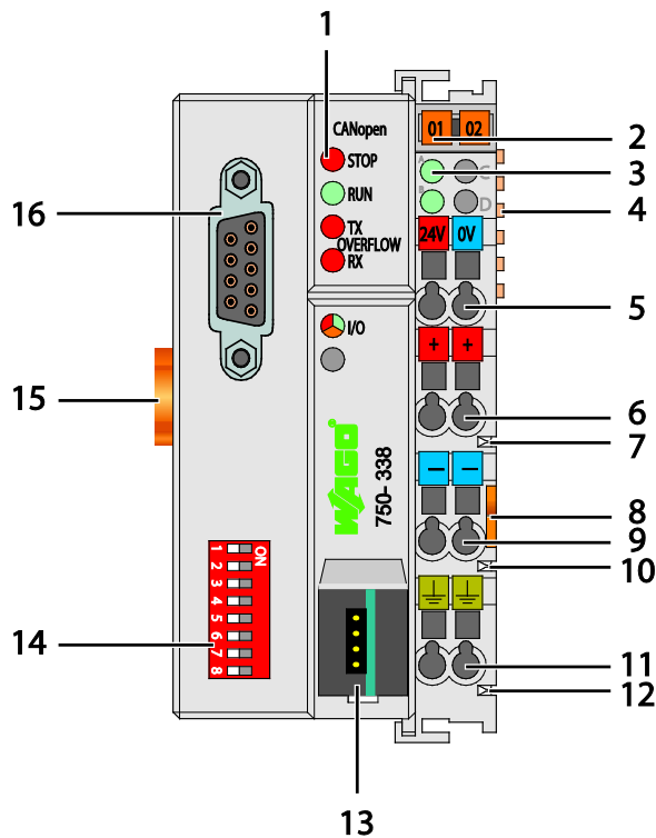
Figure 21: View CANopen Fieldbus Coupler
