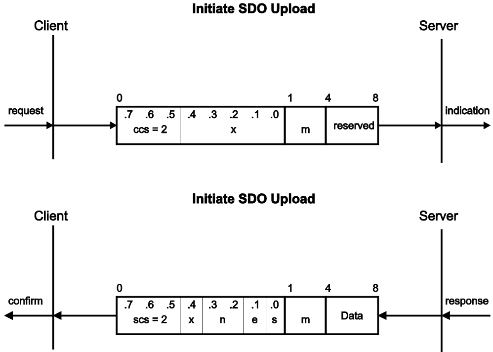
Figure 55: Initiate SDO Upload
