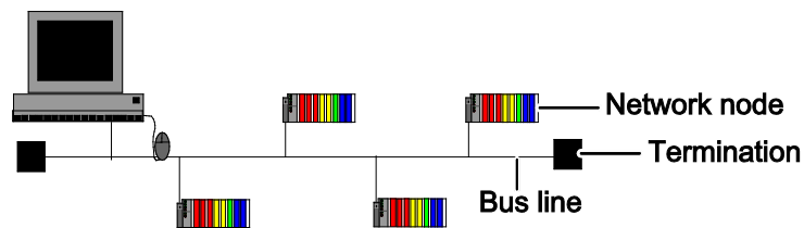
Figure 49: Bus Topology of a CANopen Network
