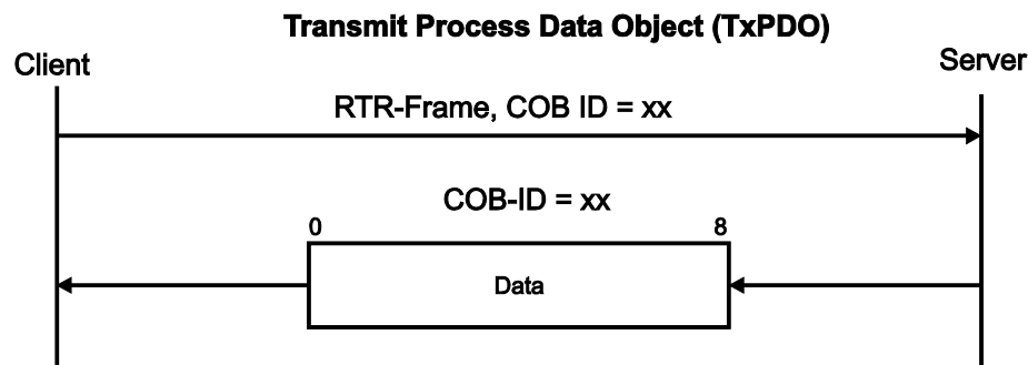
Figure 51: Tx-PDO
