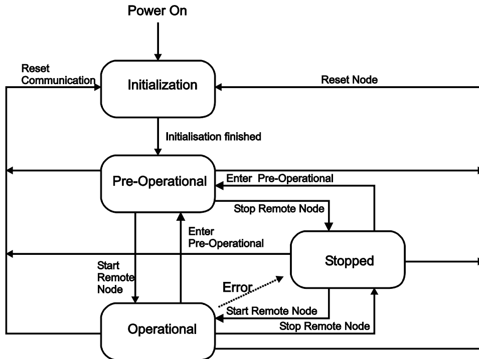
Figure 60: State Diagram of the Fieldbus Coupler/Controller
