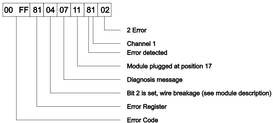
Figure 81: Structure of Emergency Telegram 2
