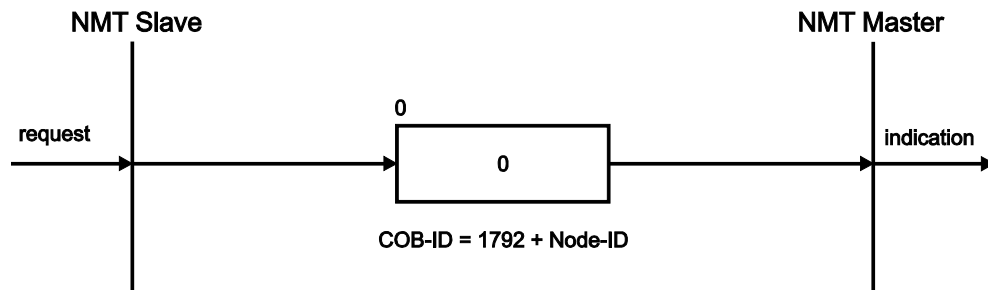
Figure 67: Bootup Protocol
