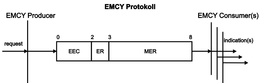
Figure 59: EMCY Protocol
