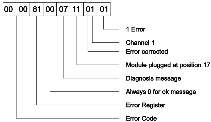
Figure 82: Structure of Emergency Telegram 3
