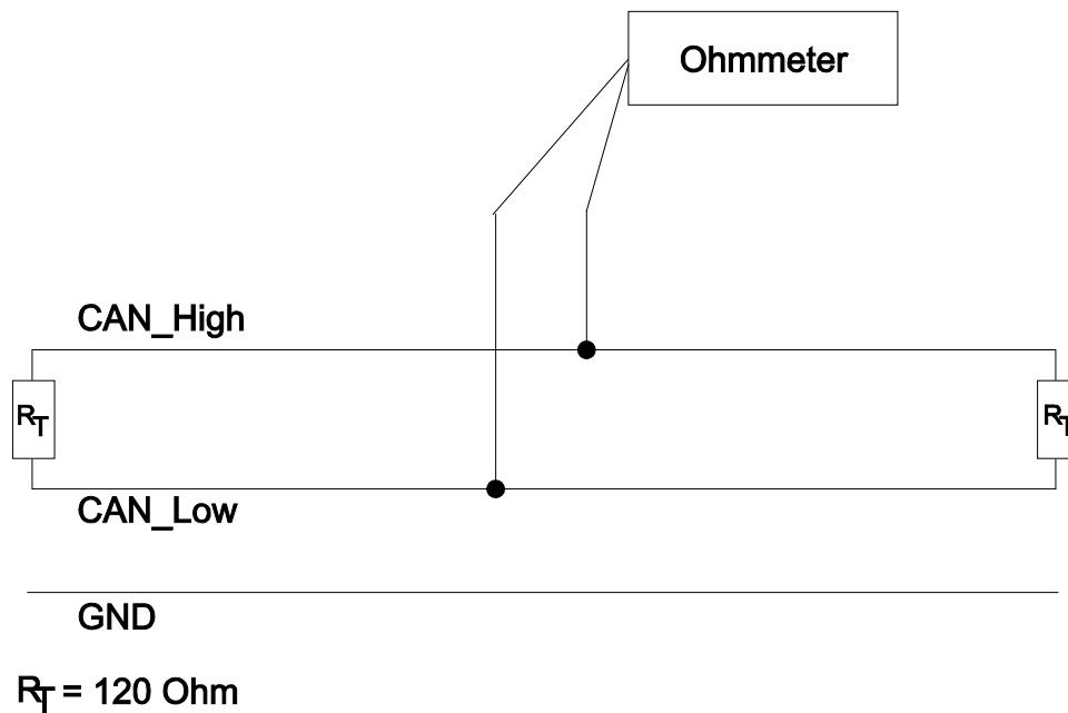
Figure 48: Principle of Measurement for Checking the CAN Bus Before Cabling
