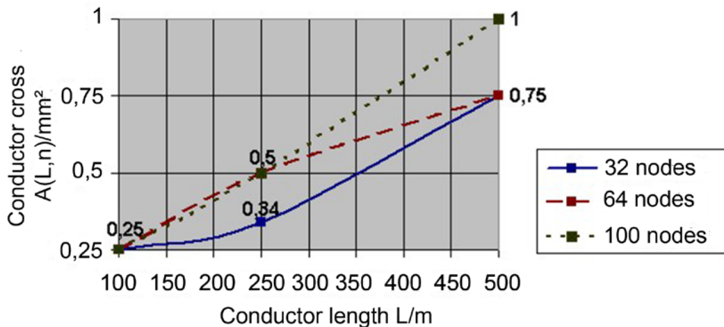
Figure 46: Cable Cross-Section Based on the Cable Length and the Number of Nodes
