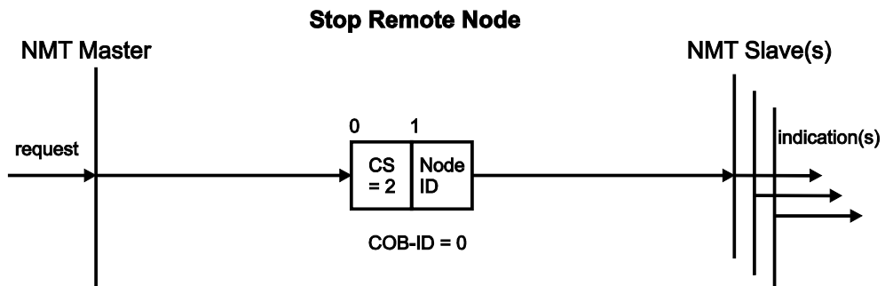
Figure 62: Stop Remote Node
