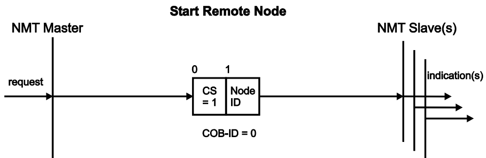
Figure 61: Start Remote Node
