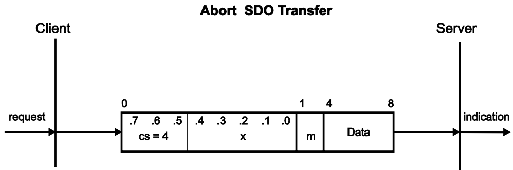
Figure 57: Abort SDO Transfer
