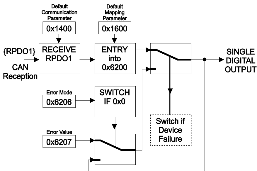
Figure 76: PDO Transmission of Digital Output Module Data
