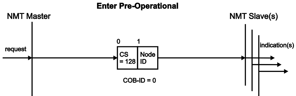
Figure 63: Enter PRE-OPERATIONAL
