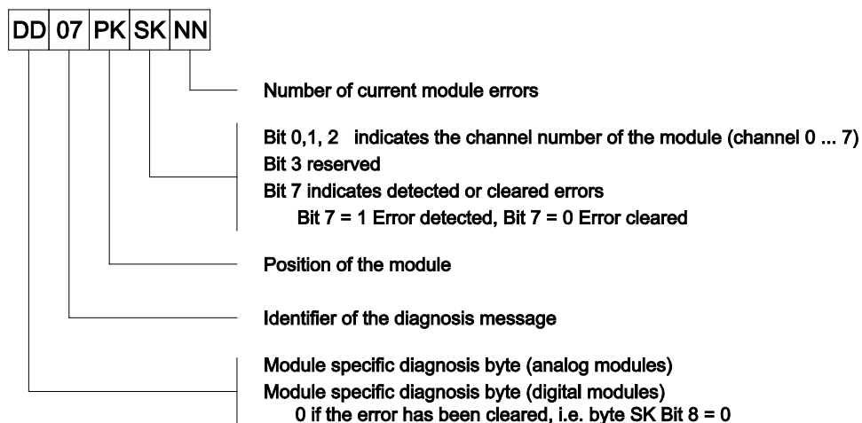
Figure 79: Structure of the “Additional Code”
