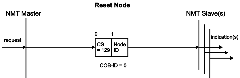
Figure 64: Reset Node
