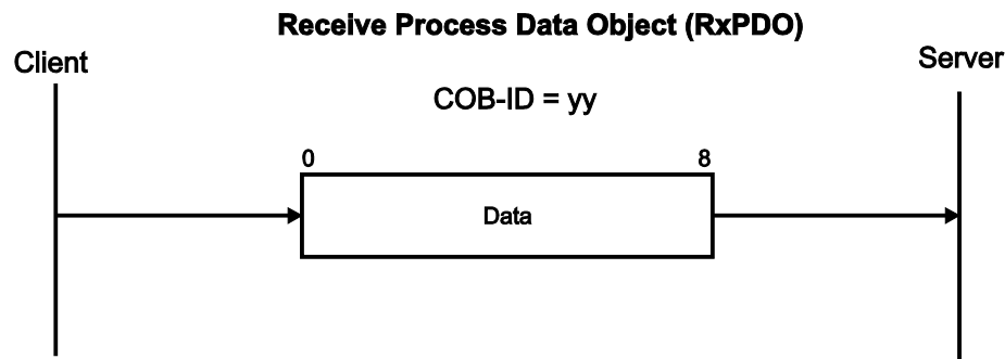
Figure 50: Rx-PDO
