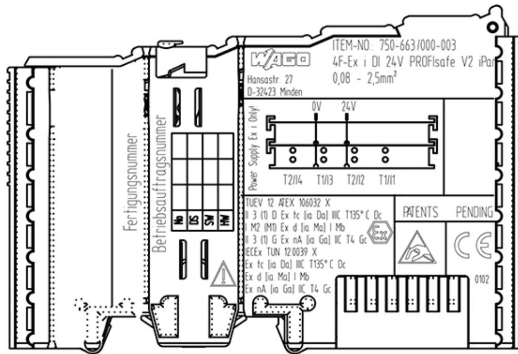
Figure 88: Side Marking Example for Approved Ex i I/O Modules According to ATEX and IECEx.
