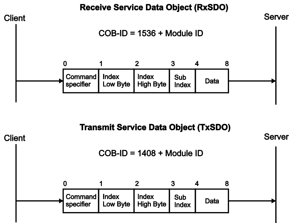
Figure 52: SDO Protocol
