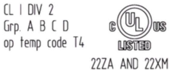
Figure 91: Text Detail – Marking Example for Approved I/O Modules According to NEC 500
