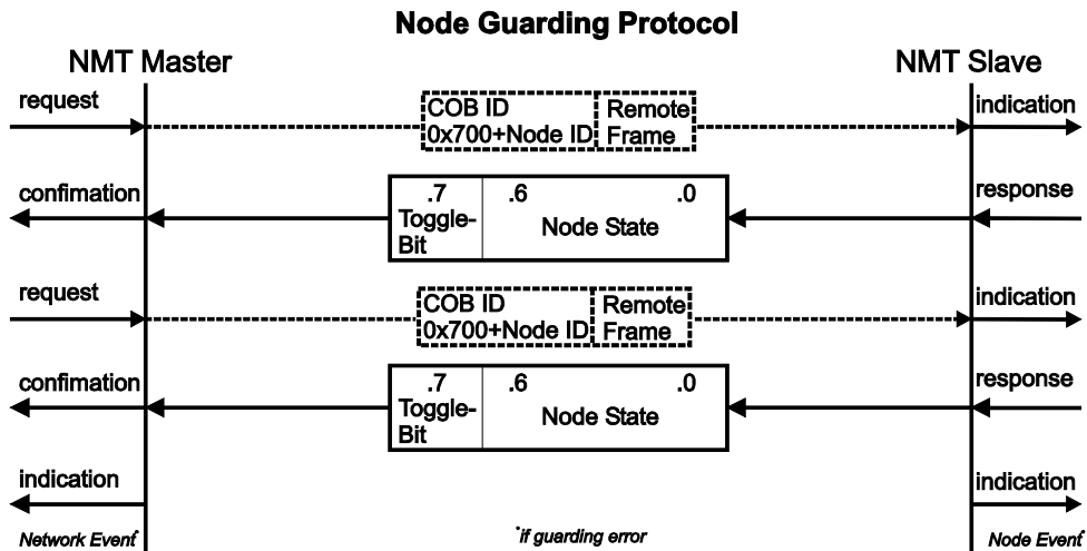
Figure 65: Node Guarding Protocol
