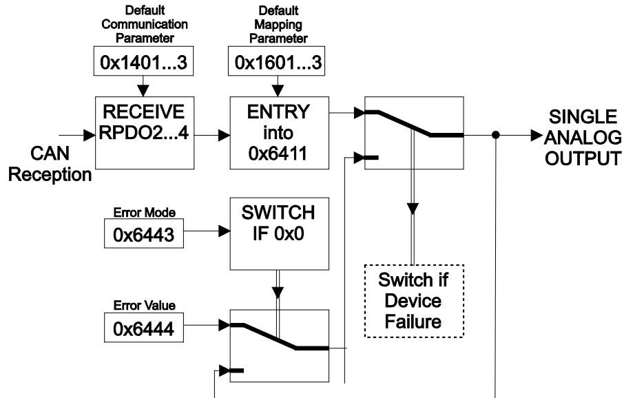
Figure 78: PDO Transmission of Analog Output Module Data
