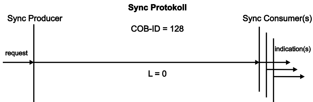
Figure 58: SYNC Protocol
