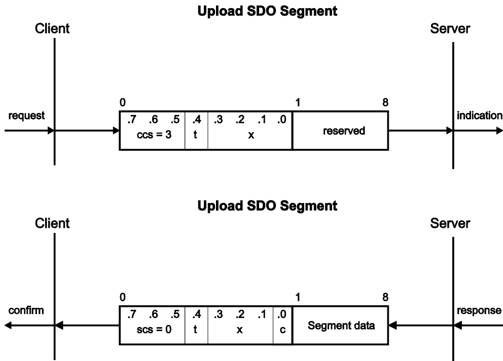
Figure 56: Upload SDO Segment
