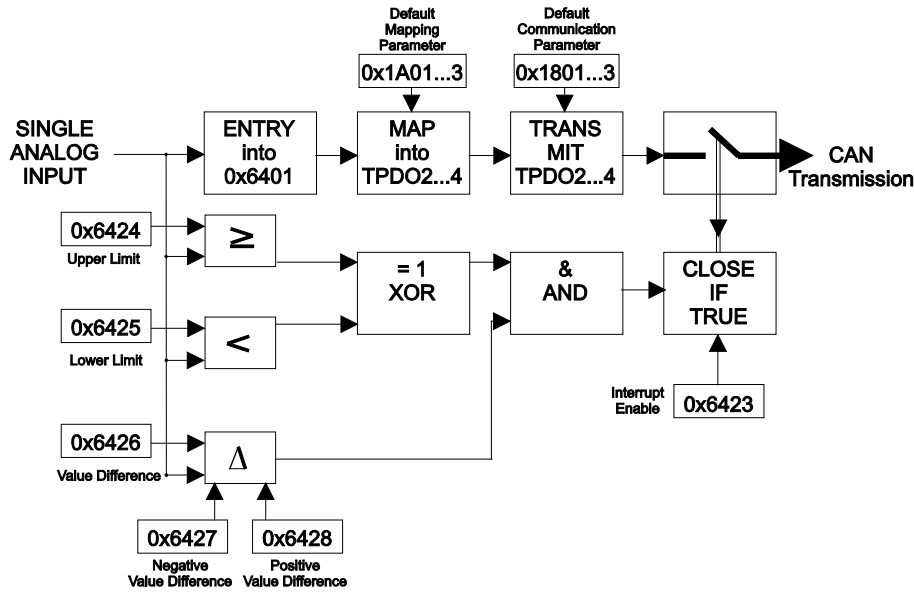
Figure 77: PDO Transmission of Analog Input Module Data
