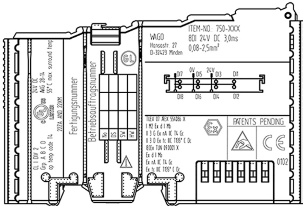
Figure 90: Side Marking Example for I/O Modules According to NEC 500
