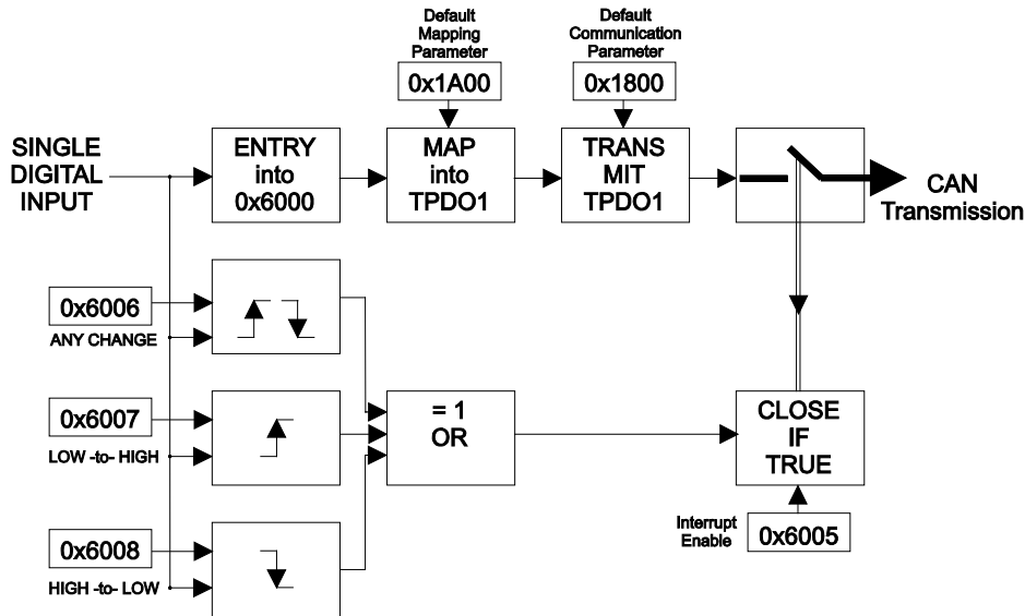
Figure 75: PDO Transmission of Digital Input Module Data
