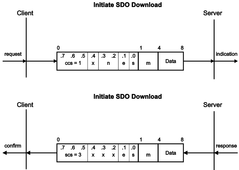
Figure 53: Initiate SDO
