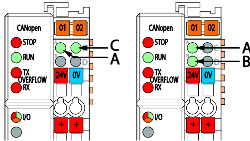
Figure 43: Display Elements
