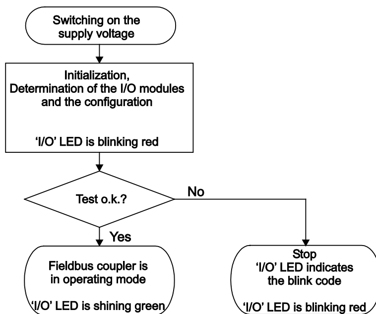
Figure 36: Operating System
