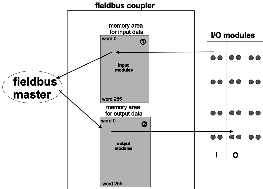
Figure 37: Memory Areas and Data Exchange
