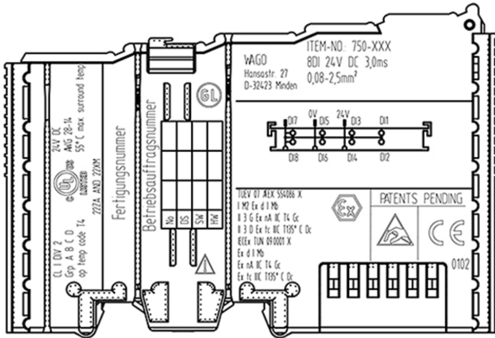
Figure 86: Side Marking Example for Approved I/O Modules According to ATEX and IECEx
