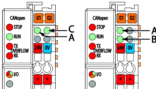
Figure 24: Display Elements
