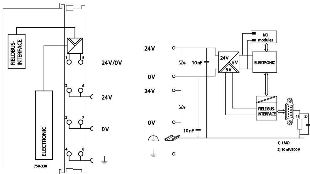
Figure 22: Device Supply
