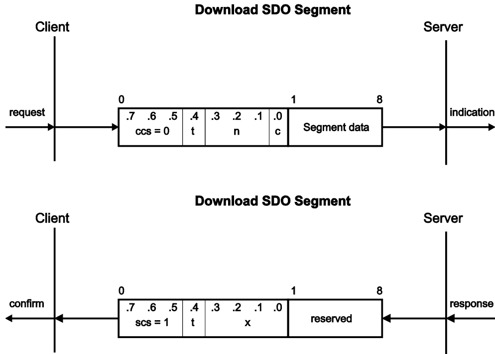
Figure 54: Download SDO Segment
