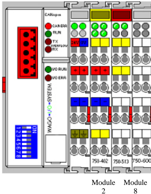
Figure 69: Example Configuration of a Node, Subset
