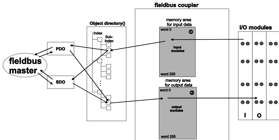
Figure 38: Fieldbus-Specific Data Exchange for a CANopen Fieldbus Coupler
