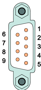
Figure 23: Pin Assignment for D-Sub Fieldbus Connection (Male)
