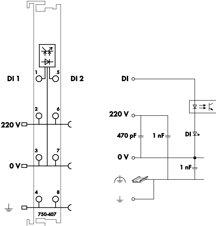
Figure 6: Schematic Diagram
