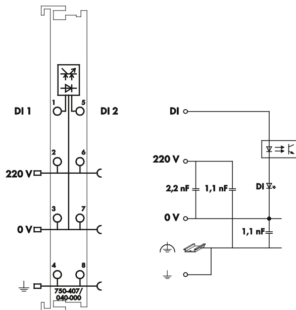
Figure 6: Schematic Diagram
