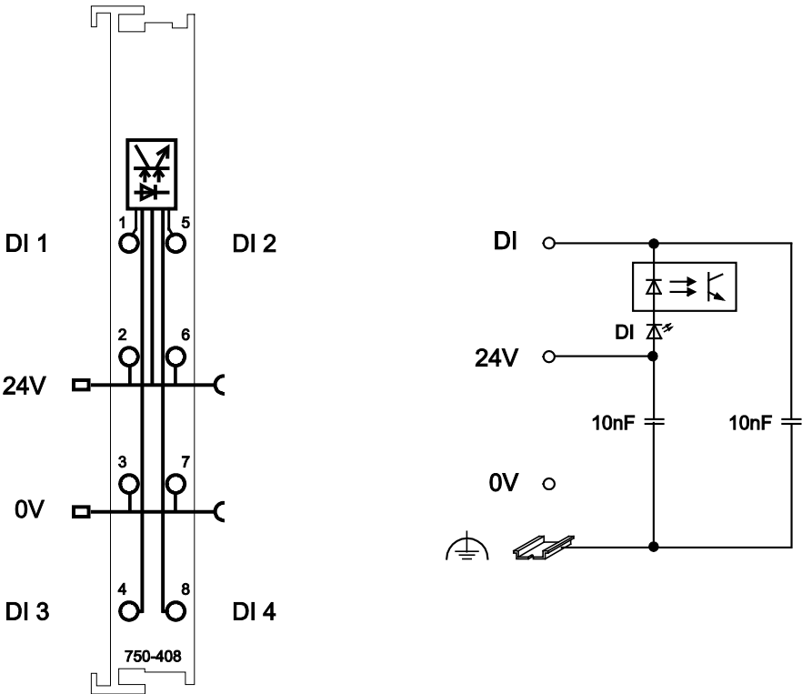
Figure 6: Schematic Diagram
