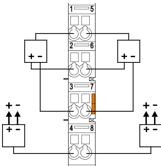
Figure 12: Connecting Diagram – 3-Conductor Connection
