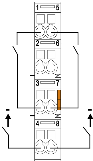
Figure 11: Connecting Diagram – 2-Conductor Connection
