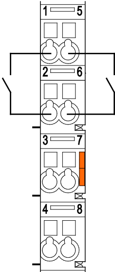
Figure 11: Connecting Diagram, 2-Conductor Connection
