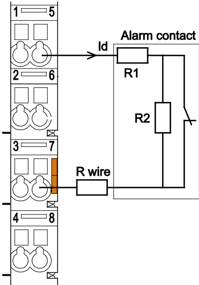
Figure 11: Connecting diagrams – 2-conductor connection
