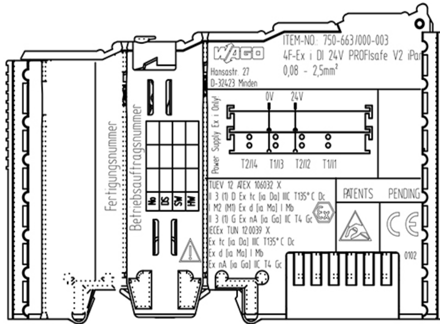
Figure 14: Side marking example for approved Ex i I/O modules according to ATEX and IECEx.
