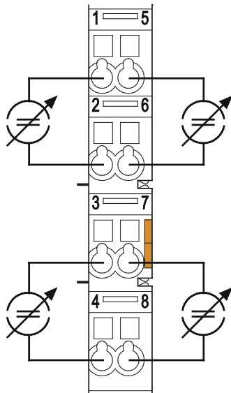
Figure 11: Connection Example
