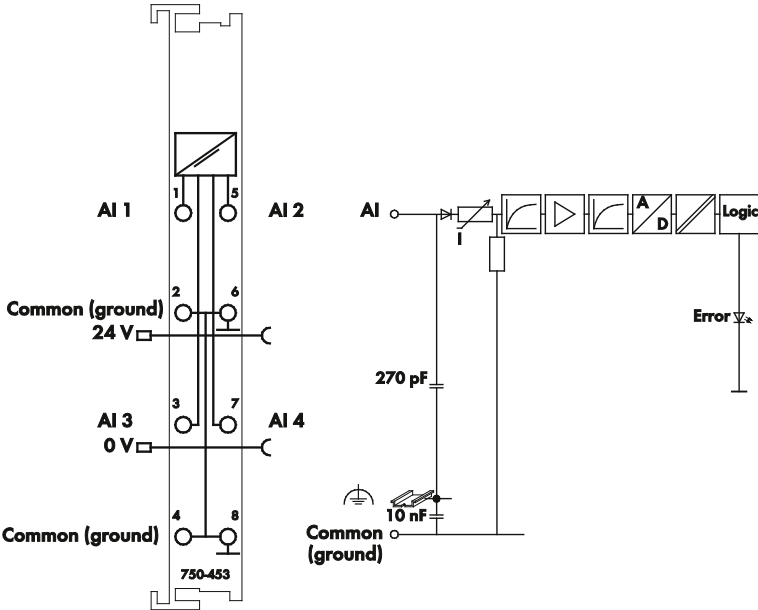
Figure 6: Schematic Diagram
