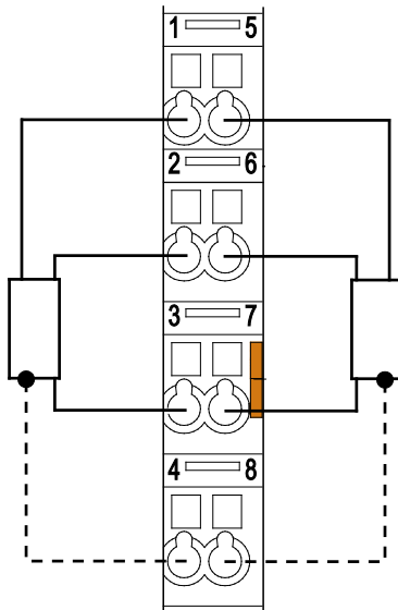
Figure 13: 3-Wire Connection 24°V
