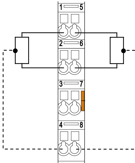
Figure 12: 2-Wire Connection 24 V
