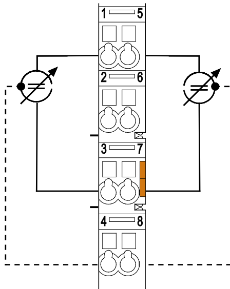
Figure 11: 2-Wire Connection 0 V
