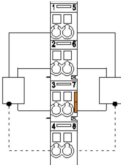
Figure 13: 3-Wire
