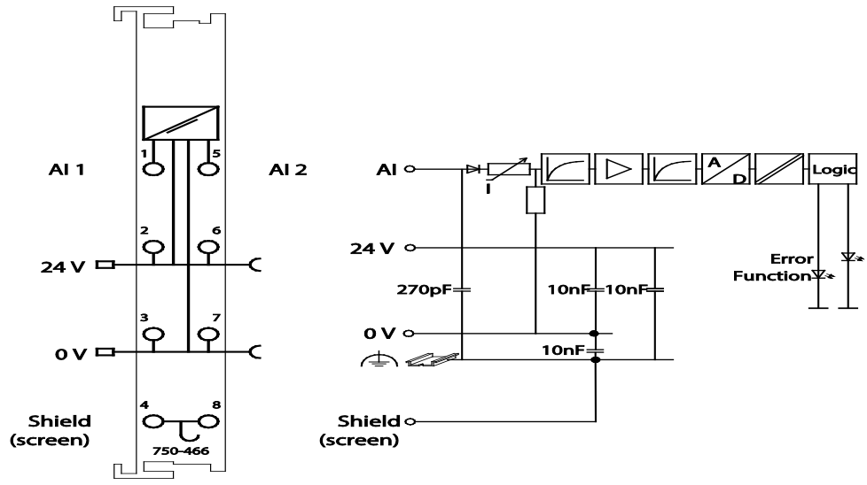
Figure 6: Schematic Diagram
