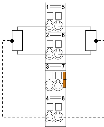
Figure 12: 2-Wire 24 V
