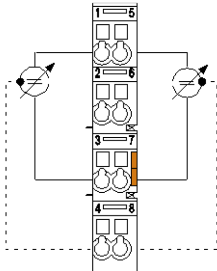
Figure 11: 2-Wire 0 V
