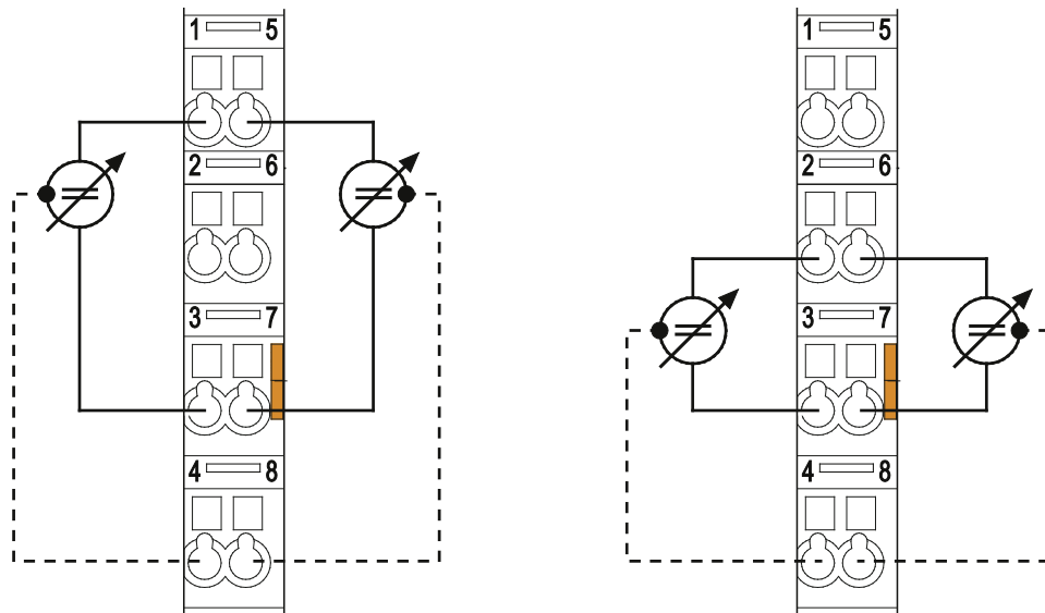
Figure 10: Connection Examples
