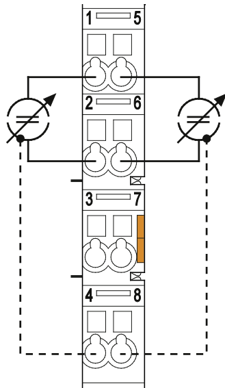
Figure 11: Connection Example
