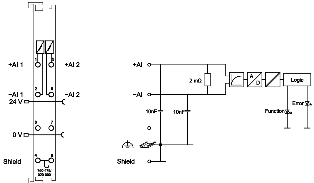
Figure 6: Schematic diagram
