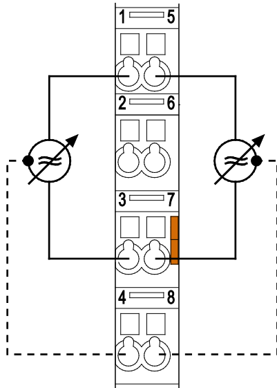
Figure 11: Connection example
