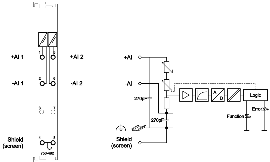
Figure 5: Schematic diagram
