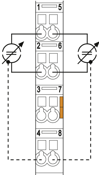
Figure 10: Connection Example 750-492
