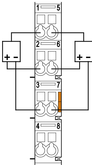
Figure 13: Connecting Diagram, 3-Conductor Connection, Ungrounded
