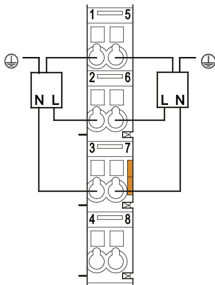
Figure 13: Connection Example, 3-Wire Connection for Protection Class I (Ground Conductor) Actuators
