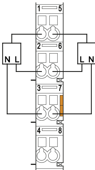
Figure 14: Connection Example, 3-Wire Connection for Protection Class II (Double Insulated) Actuators
