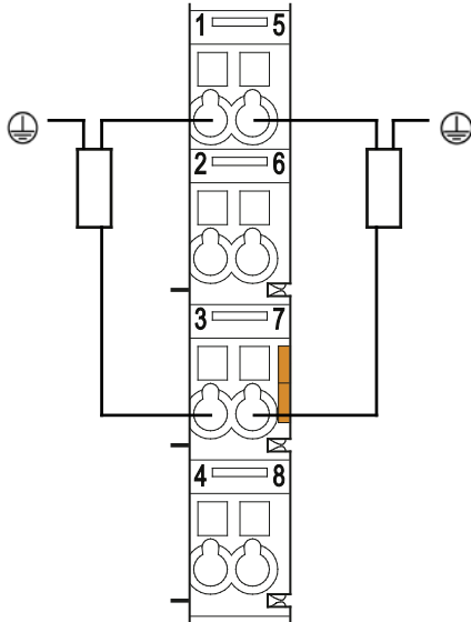
Figure 11: Connection Example, 2-Wire Connection for Protection Class I (Ground Conductor) Actuators
