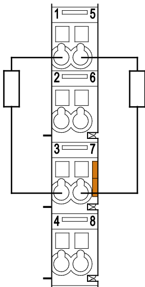
Figure 12: Connection Example, 2-Wire Connection for Protection Class II (Double Insulated) Actuators
