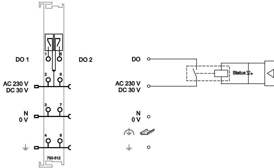
Figure 6: Schematic Diagram
