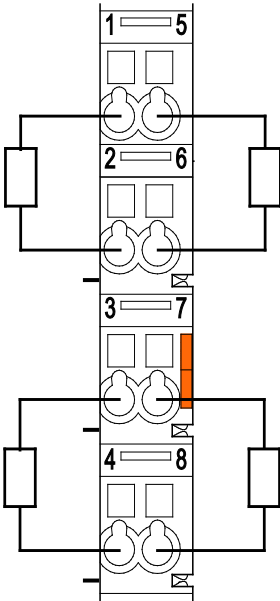
Figure 11: Connecting Diagram 2-Conductor Connection
