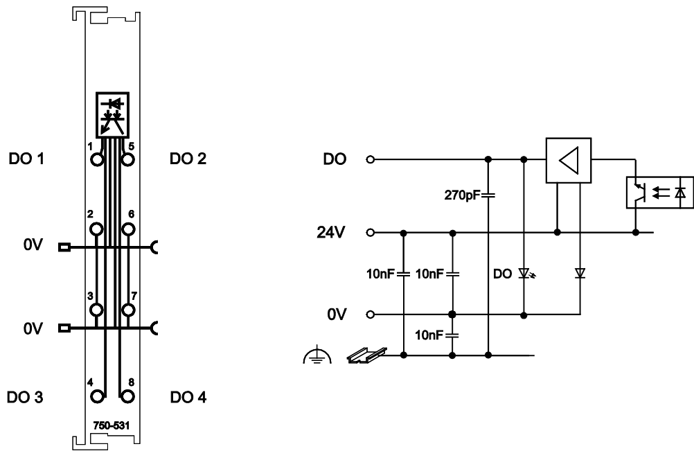
Figure 6: Schematic Diagram
