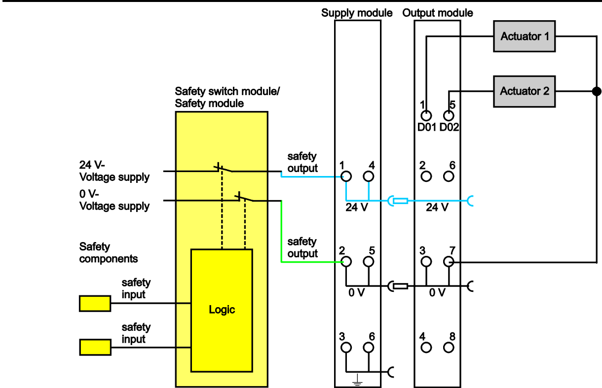
Figure 14: Two-channel Double-pole Disconnection
