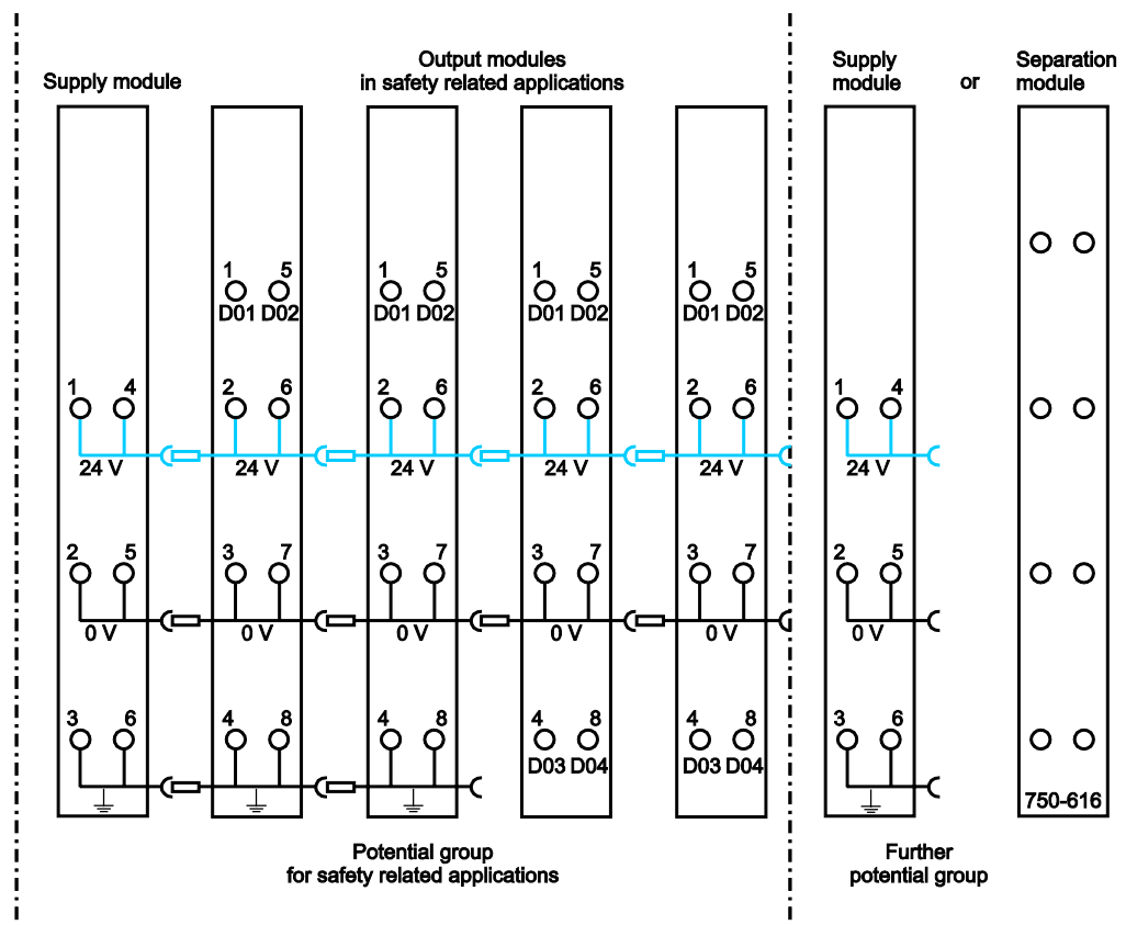
Figure 12: Potential Group for Safety Related Applications
