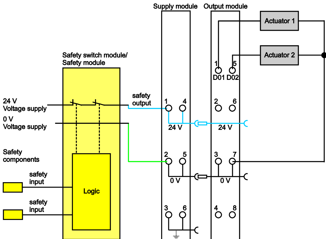
Figure 13: Two-channel Single-pole Disconnection
