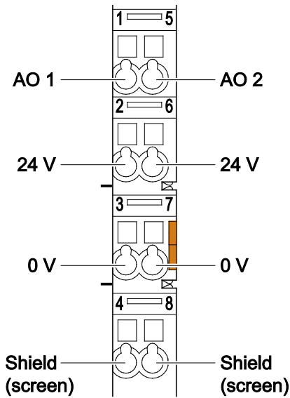
Figure 4: CAGE CLAMP® Connectors
