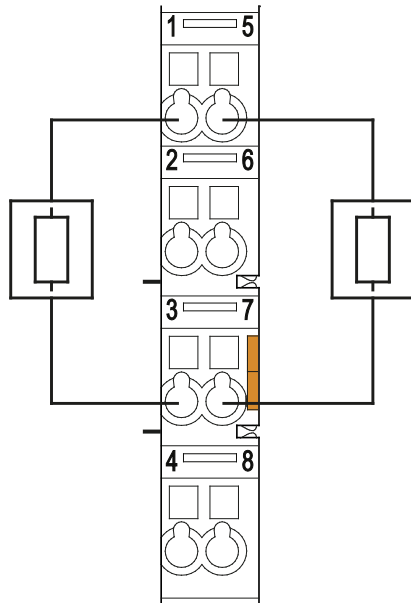
Figure 11: Connecting Diagram
