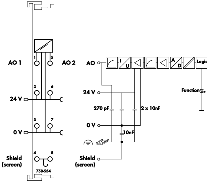
Figure 6: Schematic Diagram
