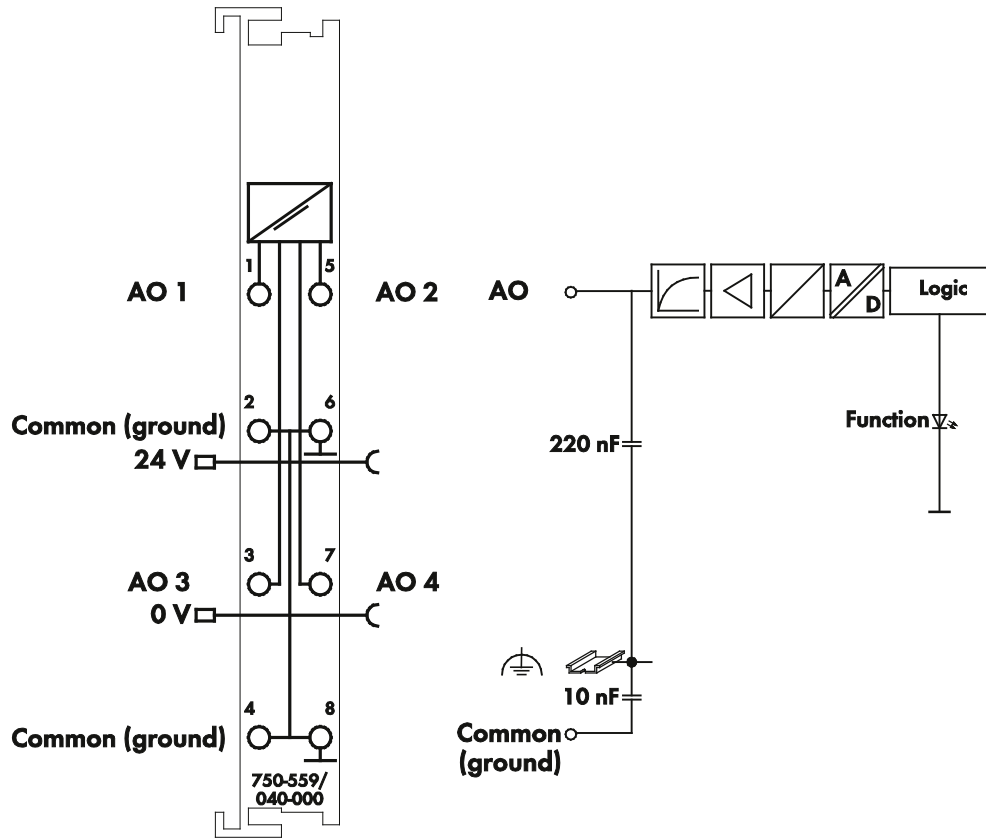
Figure 6: Schematic Diagram
