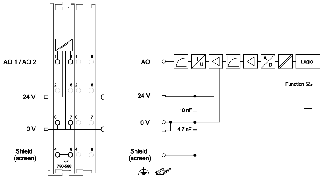
Figure 6: Schematic Diagram
