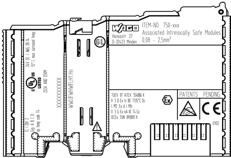
Figure 16: Marking Example According to ATEX and IECEx
