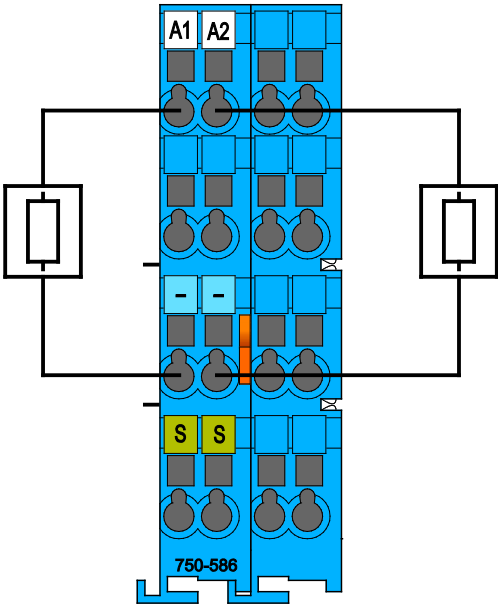
Figure 15: Connection Example
