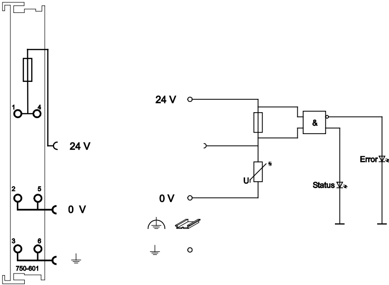
Figure 6: Schematic Diagram
