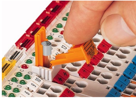
Figure 13: Opening the Fuse Holder
