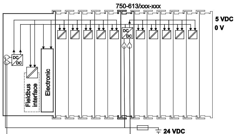
Figure 13: System Supply with an ECO Fieldbus Coupler/Controller (Supply Middle)
