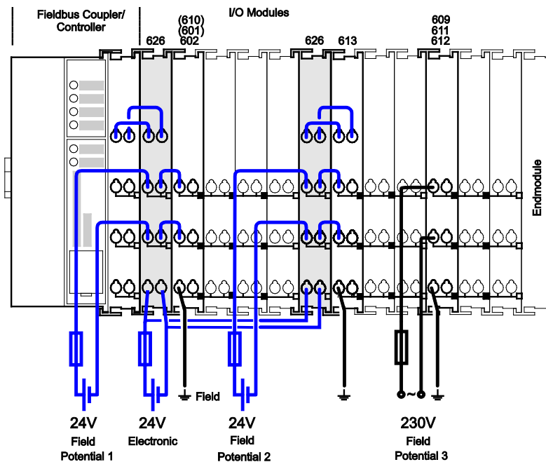
Figure 14: Power Supply Concept GL/LR
