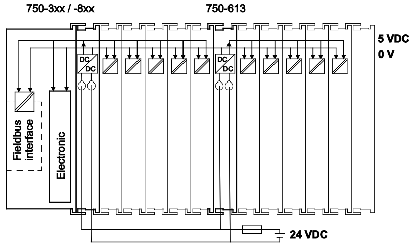
Figure 11: System Supply with a Standard Fieldbus Coupler/Controller
