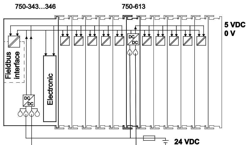
Figure 12: System Supply with an ECO Fieldbus Coupler/Controller (Supply Below)
