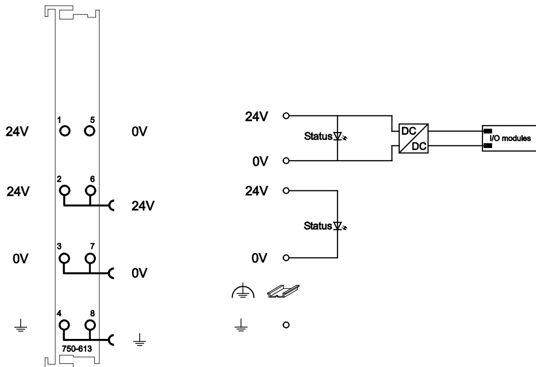
Figure 6: Schematic Diagram
