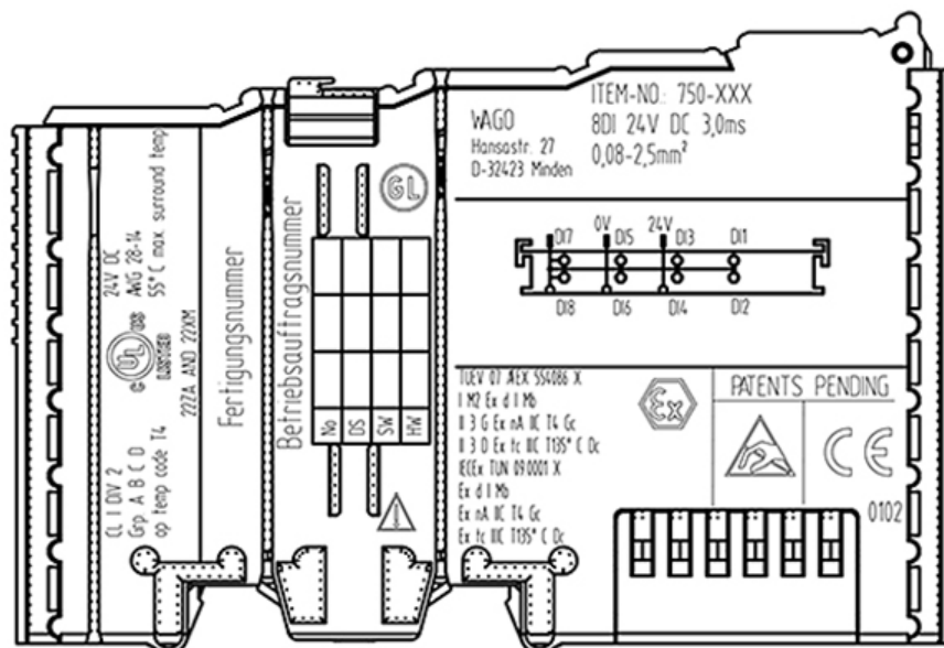
Figure 7: Side marking example for approved I/O modules according to ATEX and IECEx
