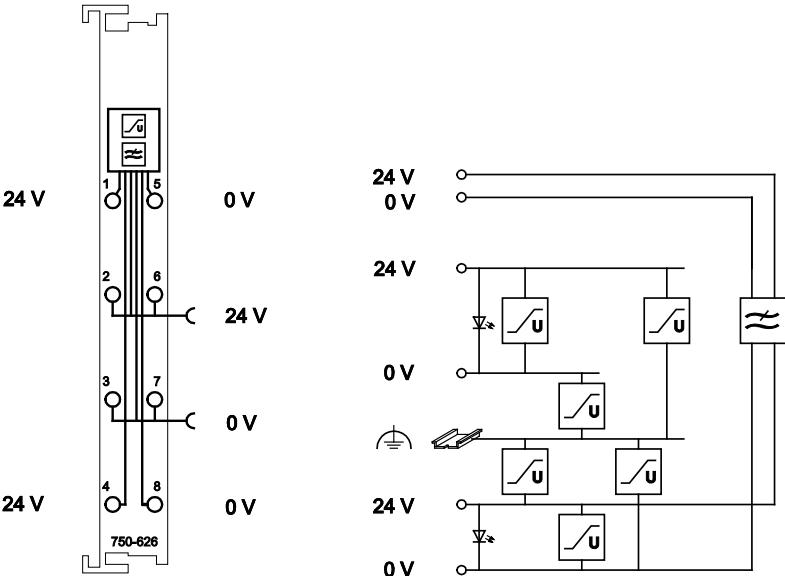
Figure 7: Schematic Diagram
