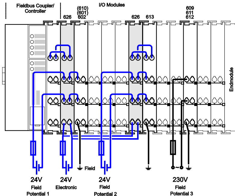
Figure 12: Power supply concept GL/LR
