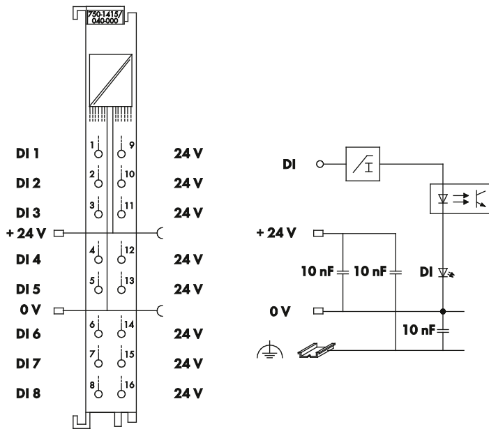
Figure 6: Schematic Diagram
