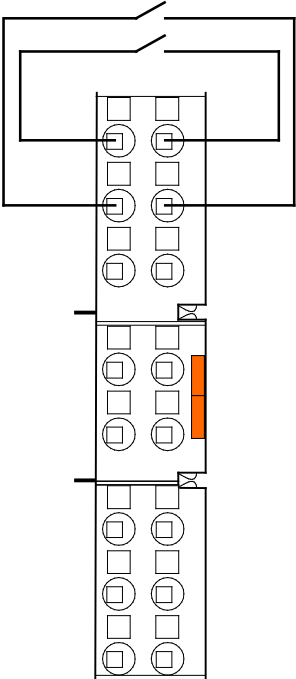
Figure 11: Connection Example with 2 Switches on Channel 1 and 2
