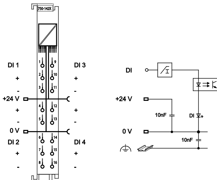
Figure 6: Schematic Diagram
