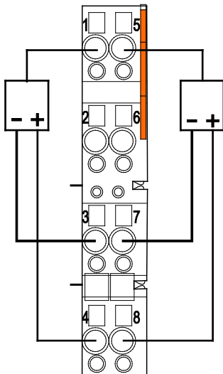
Figure 22: Connecting diagrams – 3-conductor connection
