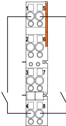
Figure 21: Connecting diagrams – 2-conductor connection
