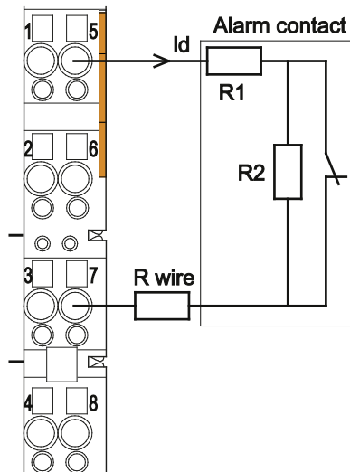
Figure 21: Connecting Diagram – 2-Conductor Connection
