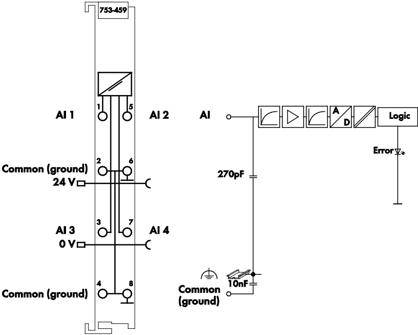
Figure 6: Schematic Diagram
