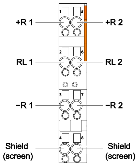
Figure 3: CAGE CLAMP® Connectors
