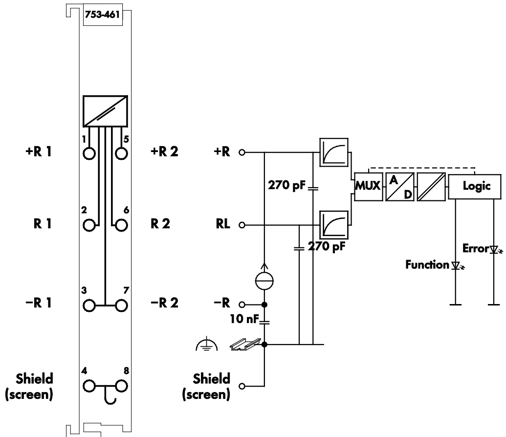
Figure 5: Schematic Diagram
