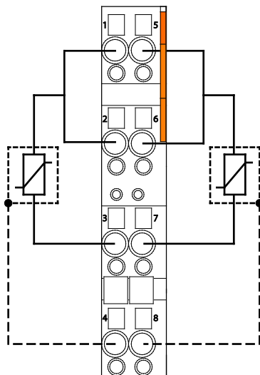
Figure 20: Connection Example: 2 × RTD, 2-Wire Connection
