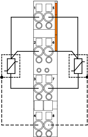
Figure 21: Connection Example: 2 × RTD, 3-Wire Connection
