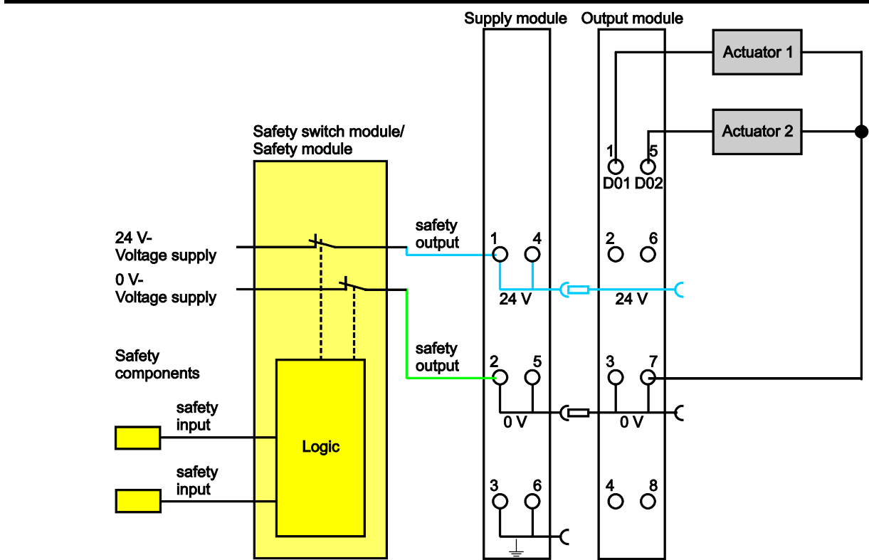
Figure 24: Two-channel Double-pole Disconnection
