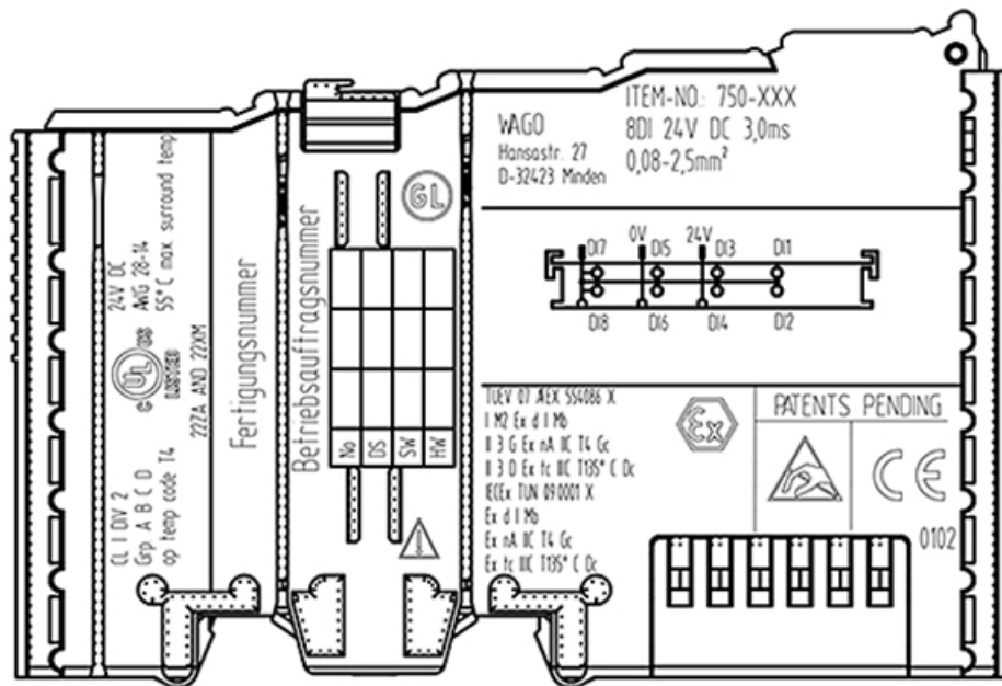
Figure 25: Side Marking Example for Approved I/O Modules According to ATEX and IECEx
