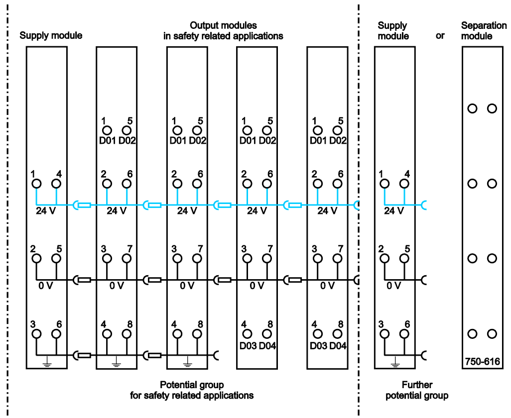
Figure 22: Potential Group for Safety Related Applications
