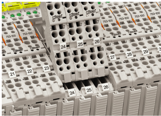
Figure 11: Assignment of Module to Connector Using Mini-WSB Tags
