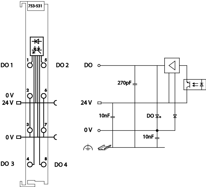
Figure 6: Schematic Diagram
