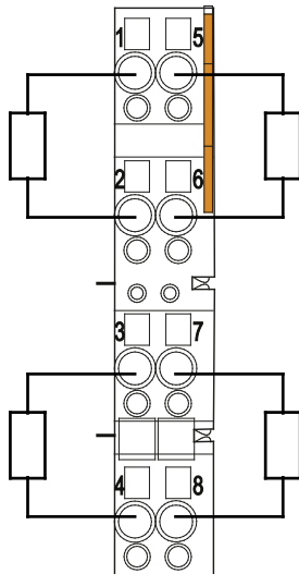
Figure 21: Connecting Diagram, 2-Conductor Connection
