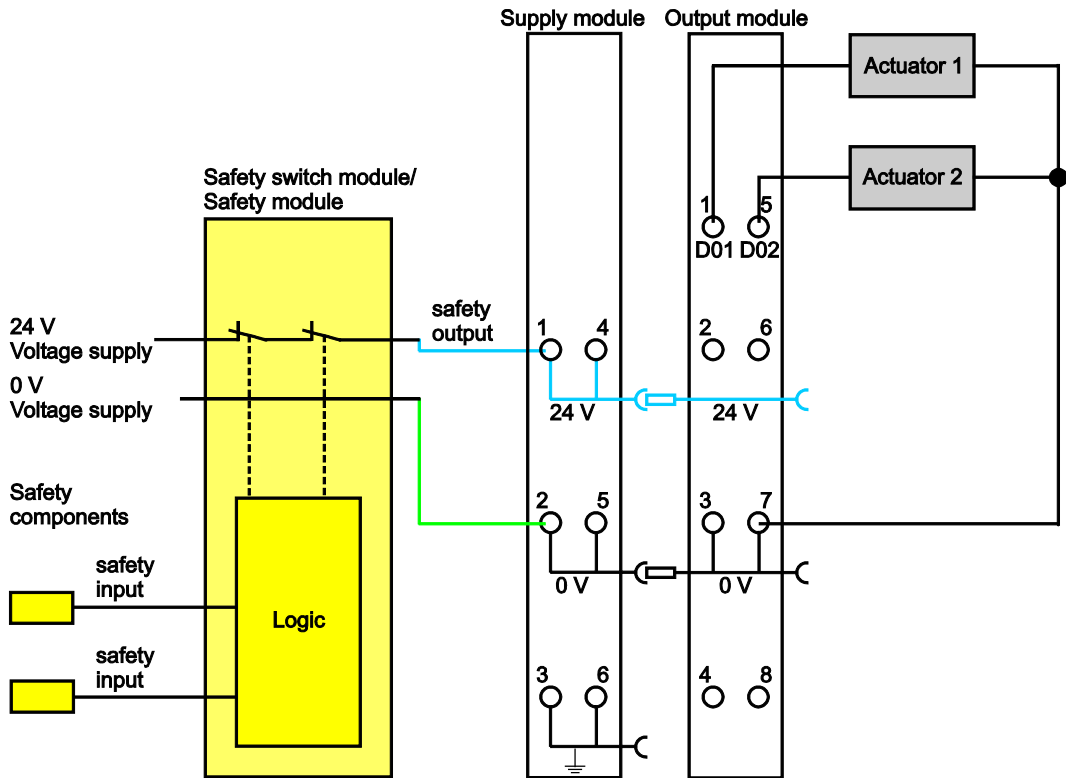
Figure 23: Two-channel Single-pole Disconnection
