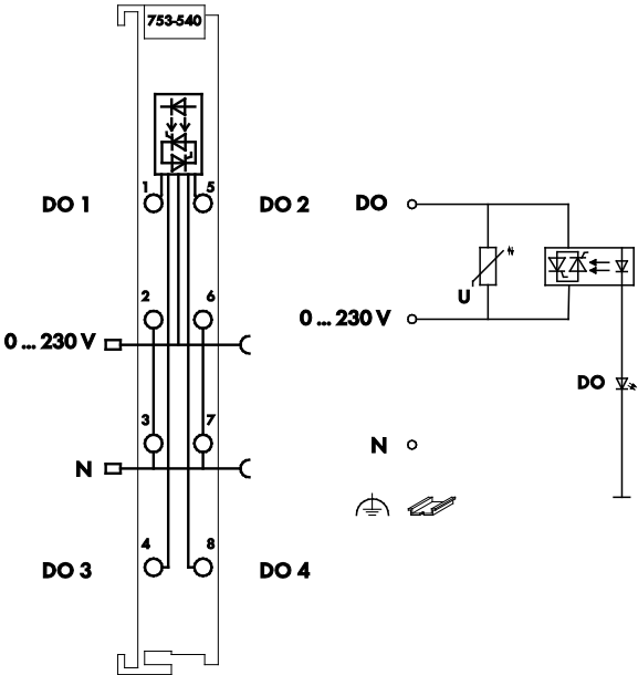
Figure 6: Schematic Diagram
