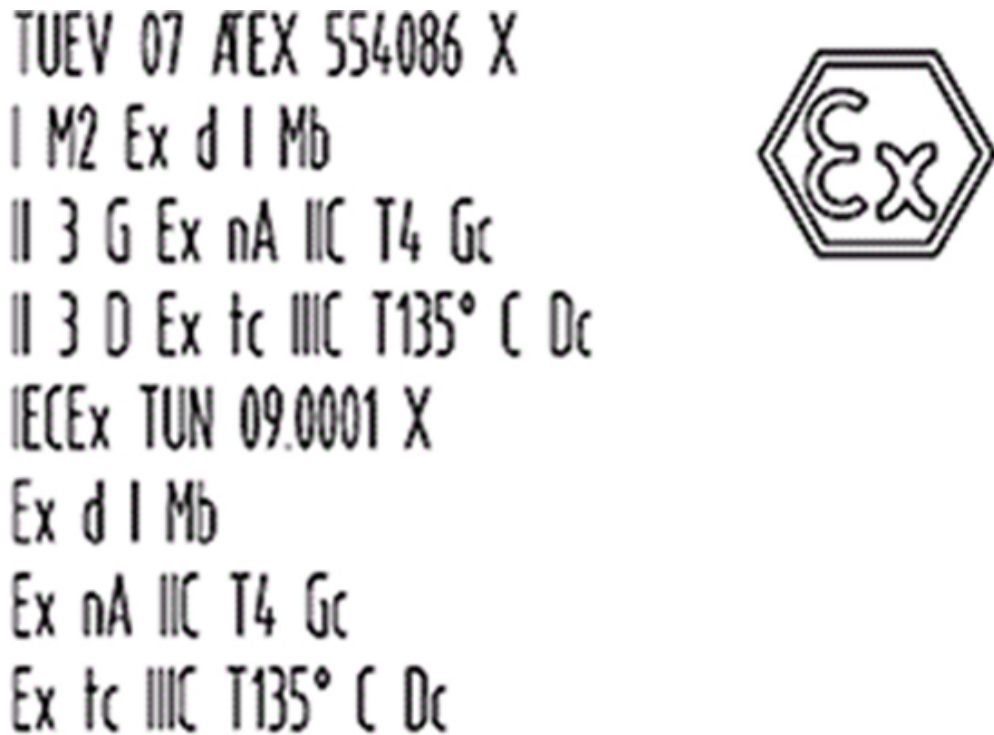
Figure 22: Text Detail – Marking Example for Approved I/O Modules According to ATEX and IECEx.
