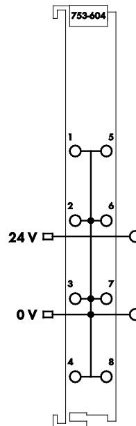
Figure 5: Schematic Diagram
